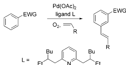
Scheme 3. Palladium-catalyzed olefination of arenes (Yu et al.).
