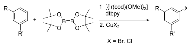
Scheme 1. Iridium-catalyzed C–H bond functionalization (Hartwig et al.). cod = 1,5-cyclooctadiene, dtbpy = 4,4'-di-tert-butyl-2,2'-bipyridine.
